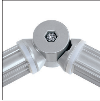
120-Degree Beam Detail
